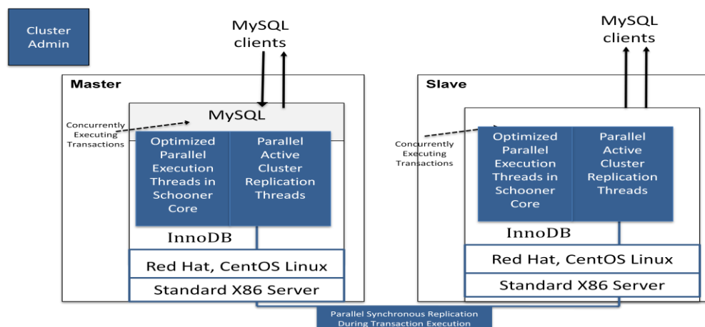
Figure 2: Tightly-Coupled Schooner MySQL Synchronous Replication Architecture
