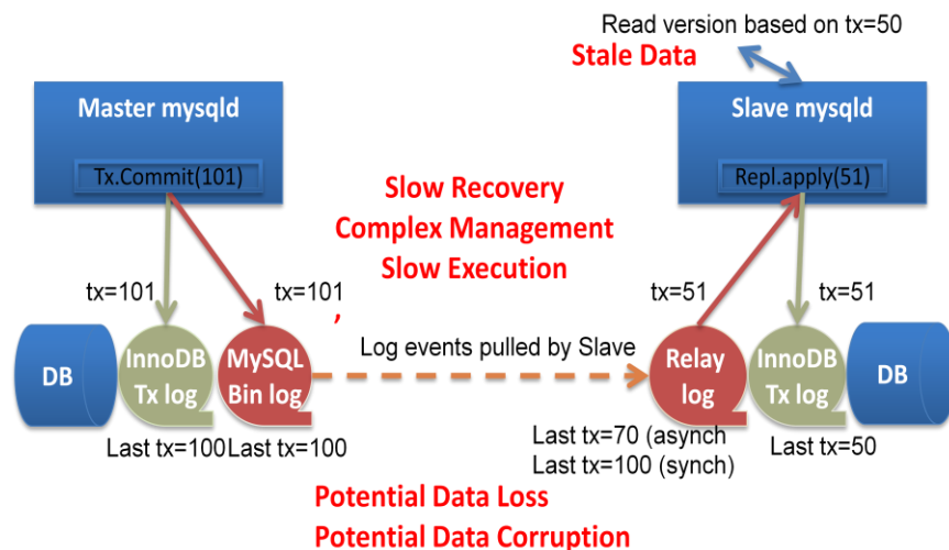
Figure 1: Loosely-Coupled MySQL Asynchronous and Semi-Synchronous Replication Architecture
