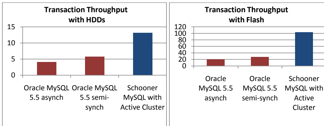
Figure 5: Synchronous Replication Cluster Performance Throughput (kTPM, 1,000 warehouses)
